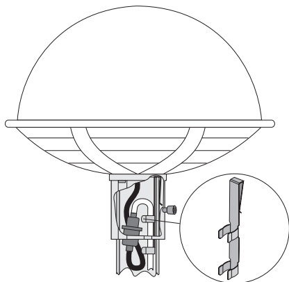
Mounting of cableholder.
