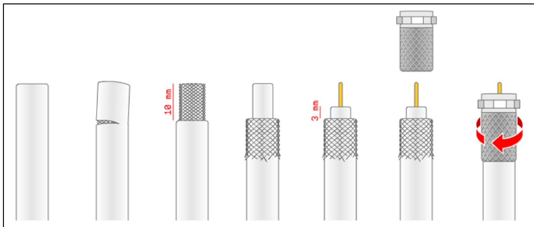
Stripping of coaxial cable for supplied twist on connectors.
